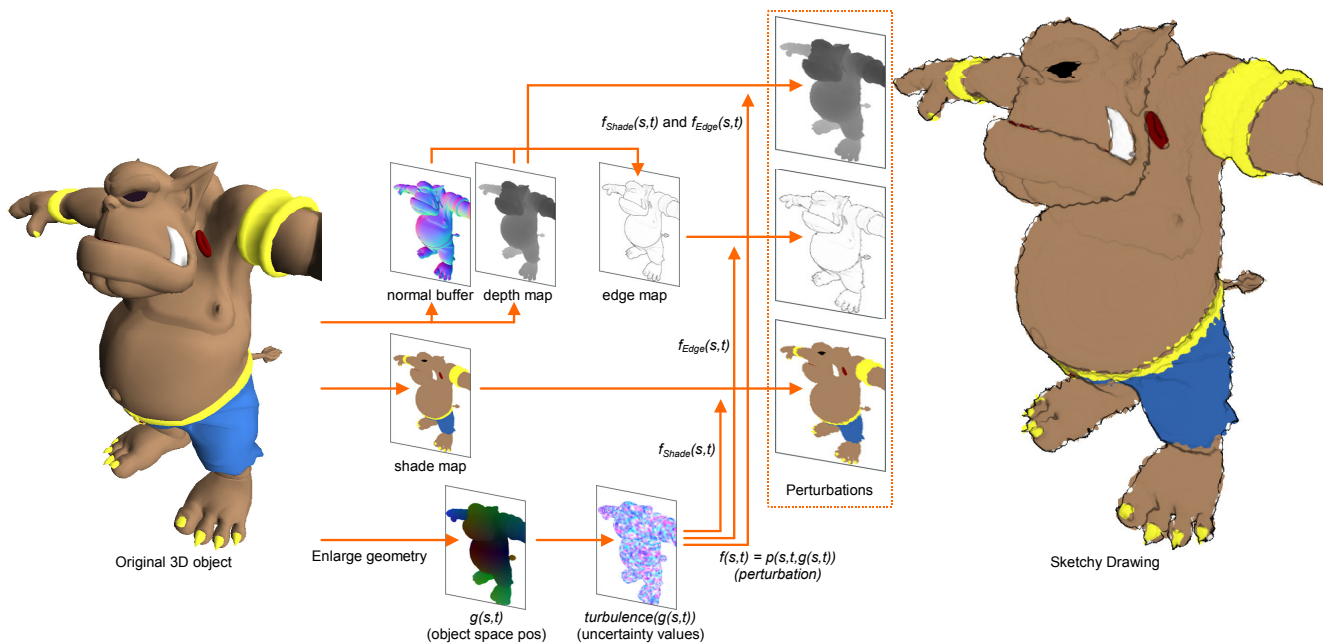
Figure 10: The conceptual sketch illustrates buffers and intermediate rendering results involved in the process of generating sketchy drawings. Furthermore, it clarifies the usage of f(s,t) when considering geometrical properties.
