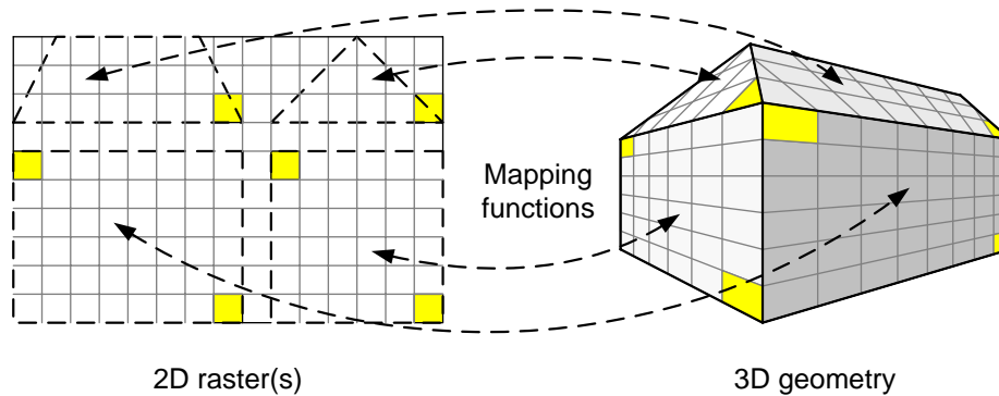
Figure 1: Schematic view of a raster-based surface property. Each surface patch is mapped to an associated unique raster area.
