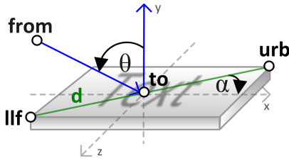
Fig. 2. Deriving the transformation using the cluster geometry and the camera properties.
