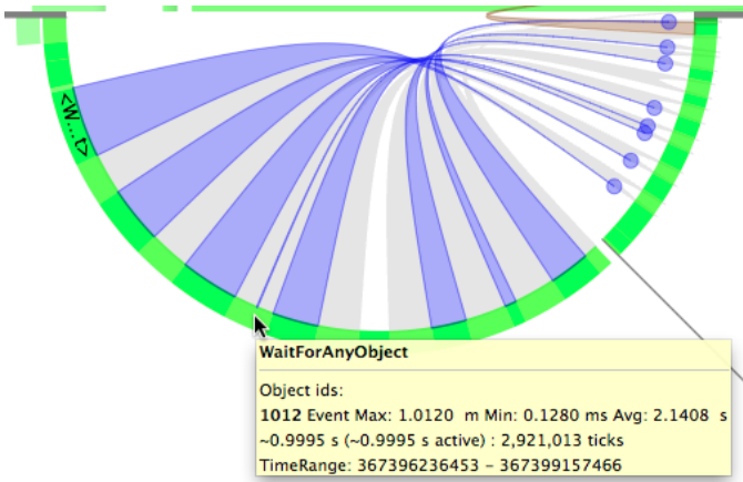
Fig. 9. The tooltip reveals which function calls are contained in the aggregation. In addition, the associated correspondence of the hovered call is displayed.
