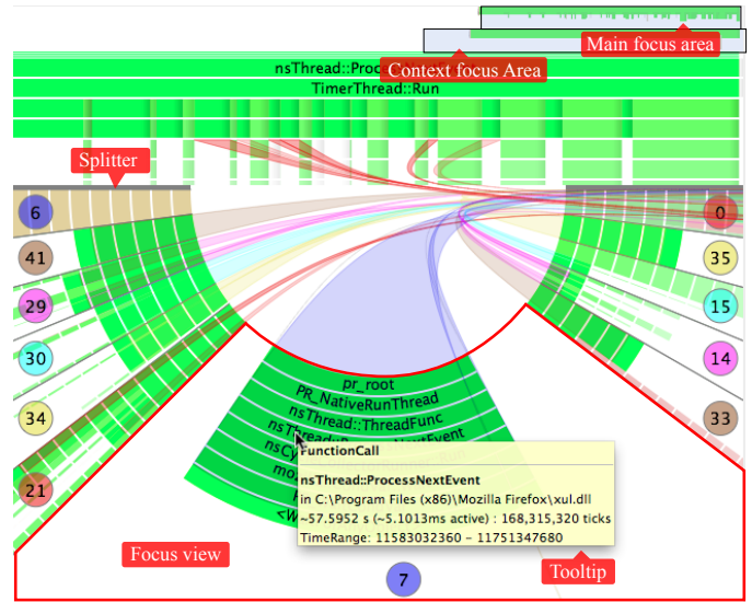
Fig. 7. 'Focusing' a thread-trace in the context view: The section of one selected thread trace on the semicircle is temporarily increased for more detailed analysis.
