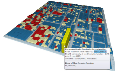
Figure 1. Treemap of a system’s static structure (courtesy of Bohnet and Döllner [3]) showing per-file outliers in max. function complexity (→ height), lines of code (→ size), and max. nesting level (→ color).
