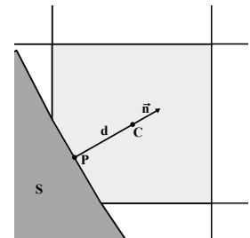
Figure 6: Computation of surface point P .
