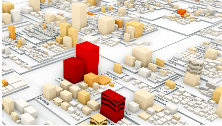
Fig. 6. A visualization result of a software system dataset. The layout was created using EvoCells layouting. The resulting visualization is a 2.5D treemap with color and height mapping, in-situ diff visualization, and labeling.
