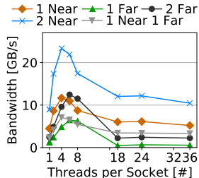
Figure 10: Writing data to Multiple Sockets.
