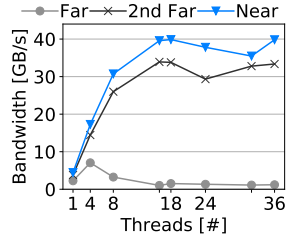
Figure 5: Read NUMA Effects.
