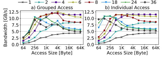
Figure 7: Write Bandwidth dependent on Access Size and Thread Count. Bandwidth is heavily impacted by the combination of access size and thread count.
