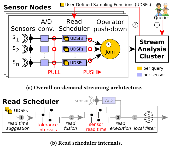
Figure 4: On-demand streaming architecture.
