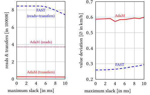
Figure 14: AdaM and FAST on football data with varying read time slack. (a) Reads & Transfers (b) Value Deviation
