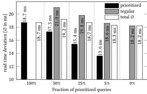
Figure 12: Query prioritization with penalty functions. (20 queries; ∅sampling rate 1Hz/-query; ∅tolerance ±0.04s)
