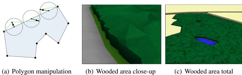
Figure 4: Abstract representations of wooded areas are created by adding and moving additional points on polygon (a) and extruded surface (b). Contained water areas are cut out of the polygon (c).
