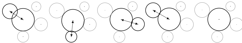
Figure 13: The example shows how the displacement works: overlapping landmarks are shifted in regard to each other iteratively. This is repeated until no more overlapping occurs or a maximum of iterations is reached.
