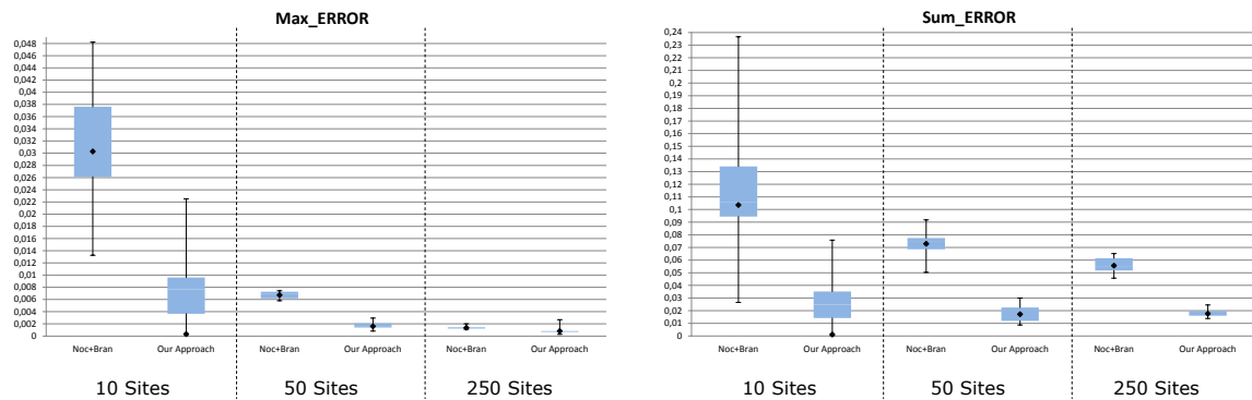
(a) Maximum target error rates
