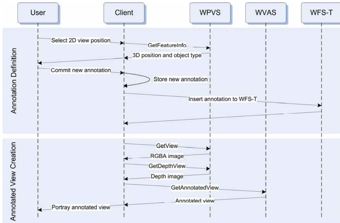
Figure 5: Sequence diagram describing the overall workflow for defining and creating the annotated perspective view.
