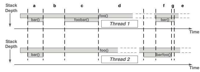
(b) Partial order-preserving scaling: All selected threads' timestamped events are merged into a single queue. Timestamp differences (a, b, c, ...) are now calculated based on the merged queue.
