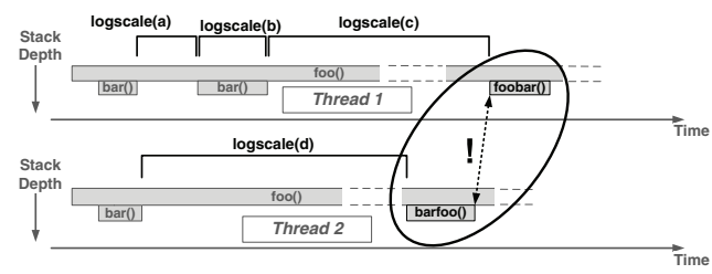
(a) Logarithmic scaling per thread. The execution of foobar() in thread 1 is no longer depicted as concurrent to the execution of barfoo() in thread 2.
