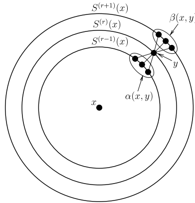
Fig. 1. Illustration of approaching set \alpha(x, y) and retreating set \beta(x, y) . For some y with \mathcal{D}(x, y) = r .
