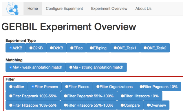
Figure 2: New dataset filter buttons for A2KB experiments.
