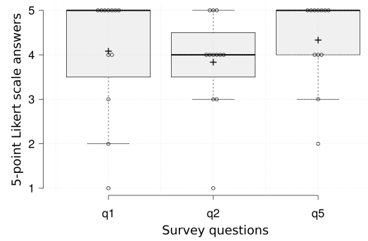
Fig. 3. Summary of answers to Likert-scale questions 1, 2 and 5 as a box plot. Center lines show the medians, box limits indicate the 25th and 75th percentiles. Whiskers extend 1.5 times the interquartile range from the 25th and 75th percentiles, outliers are represented by dots. Crosses represent sample means, data points are plotted as open circles. N = 12.
