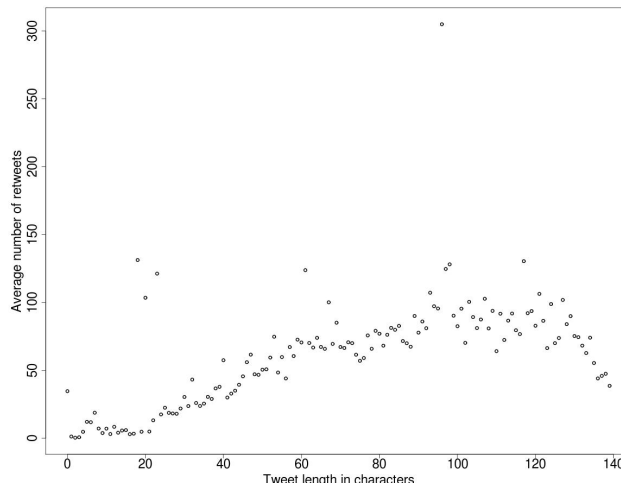
Figure 2: Average number of retweets in relation to the tweet length.
