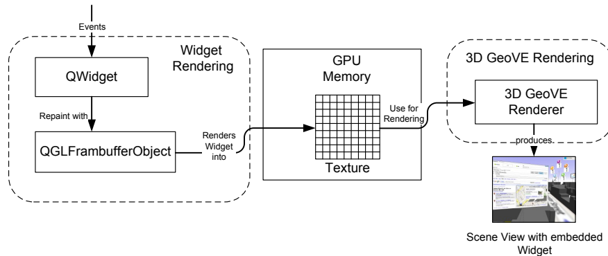
Fig. 5. Process of efficiently rendering an embedded widget. A QGLFramebuffer-Object is used as rendering device for the Qt widget. An OpenGL texture in GPU memory is used as render target. No separate transfer of pixel data to the GPU for rendering of the 3D GeoVE is necessary.
