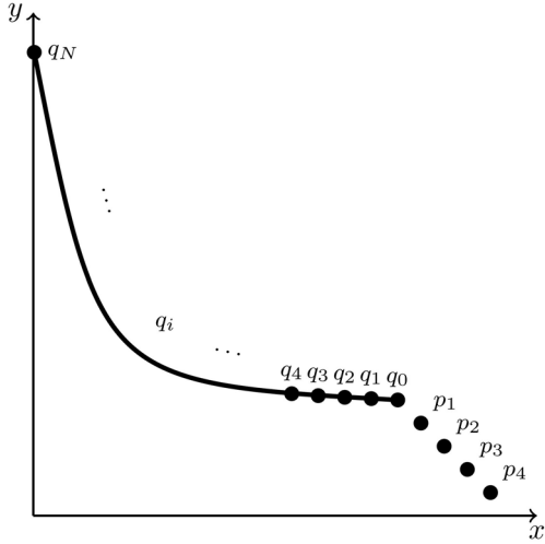
Fig. 2. Illustration of the proof of Theorem 10.
