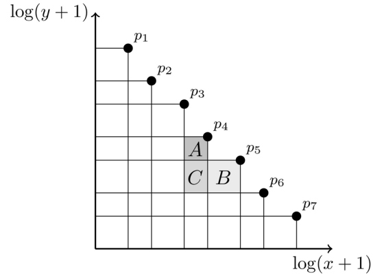
Fig. 1. Schematic log-log plot of the example used in the proof of Theorem 6. The considered areas A, B, C are indicated.
