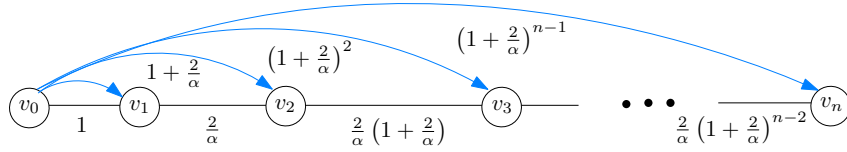
Figure 9: Lower bound graph. The black graph corresponds to the social optimum P_{n+1} , the blue graph S_{n+1} is in NE.
