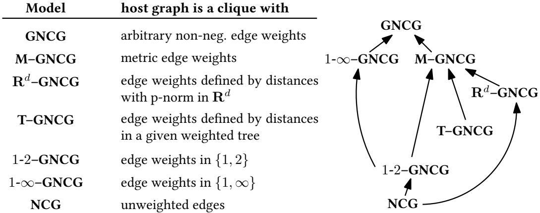
Figure 1: Left: Model overview. Right: Model relations. Arrows point from special case to more general model.
