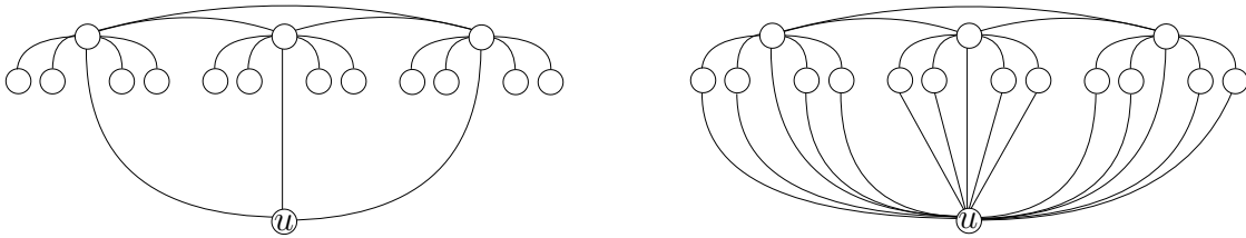
Figure 3: NE and optimal networks. All depicted edges are 1-edges. On the right hand side, the optimal network for \alpha = 1 is depicted. The graph on the left hand side is a NE for every 1/2 \leq \alpha \leq 1 .
