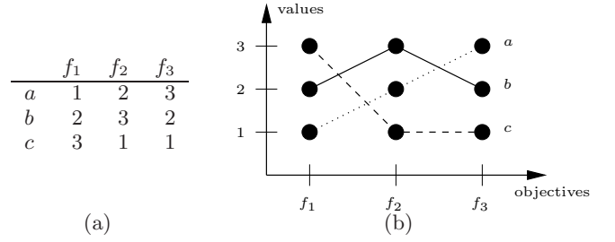
Figure 1: Objective values (a) and corresponding parallel coordinates plot (b) for three solutions a, b, c \in X .
