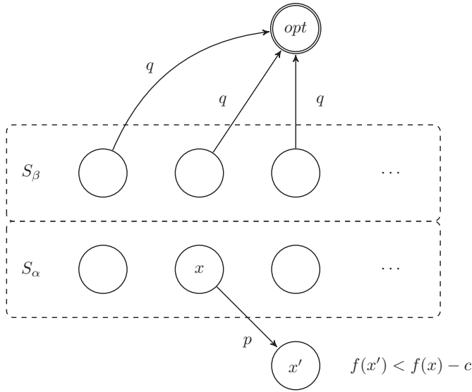
Figure 4: Partitioned Markov chain with transition probability bounds. S_\alpha contains all states corresponding to tours that have intersecting edges. S_\beta contains all states corresponding to suboptimal intersection-free tours. Note that x' can be in either S_\alpha or S_\beta .
