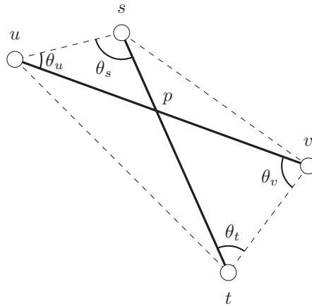
Figure 1: Edges that intersect at a point p form the diagonals of a convex quadrilateral in the plane. Interior edges define nondegenerate triangles with given angles.
