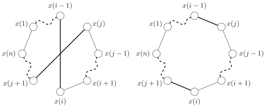
Figure 2: The effect of the inversion \sigma_{ij}^I operation on a Hamiltonian cycle. Inverting a subsequence in the permutation representation corresponds to a 2-opt (or 2-change) move in which a pair of edges in the current Hamiltonian cycle are replaced by a pair of edges not in the current cycle.
