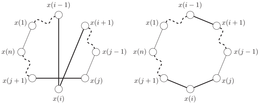
Figure 3: The effect of the jump operation \sigma_{ij}^J on a Hamiltonian cycle.
