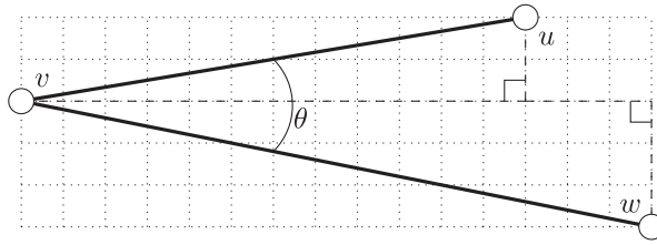
Figure 7: If the slope of the lines from v to u and v to w are of opposite sign, they form the hypotenuses of two right triangles and \theta \geq 2 \arctan((m - 1)^{-1}) .
