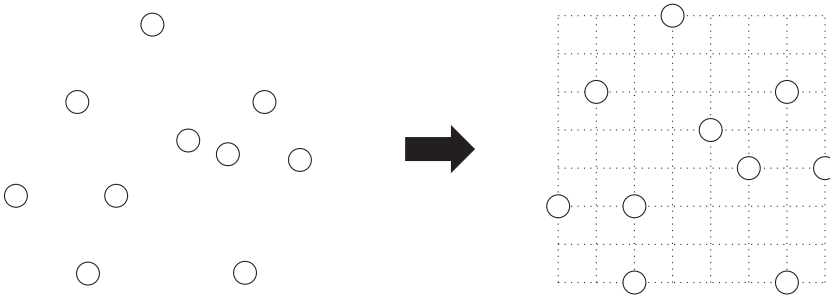
Figure 5: Quantizing a set of n points in the plane onto an m \times m grid. Coordinates are rounded to the nearest value in a set of m equidistant values.
