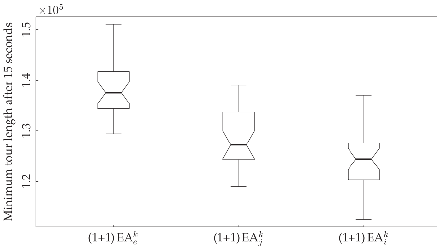
Figure 6: Comparison of solution quality (minimum tour length values) of (1 + 1) EA_e^k , (1 + 1) EA_i^k , and (1 + 1) EA_j^k obtained within 15 s on 30 instances of size 100 and inner point percentage 40.
