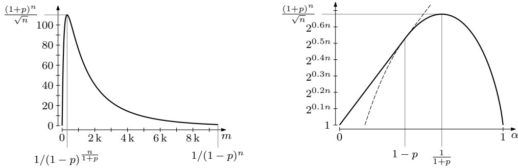
(a) Our bound as a function of m for n = 10 and p = 0.6 in the information-theoretic regime. The vertical line at m = 1/(1-p)^{\frac{n}{1+p}} indicates the maximum (Theorem 2). For m > 1/(1-p)^n , the size goes to 1. The linear bound for m \leq 1/(1-p)^{(1-p)^n} is not shown as it is too close to 0. (b) Our bound as a function of \alpha for p = 0.6 (the plot is independent of n ). The vertical line at \alpha = 1/(1+p) indicates the maximum (Theorem 2). For \alpha \leq 1-p , the linear bound holds, for larger \alpha , we get the information-theoretic bound. They are continued as dashed lines into the other regime.
