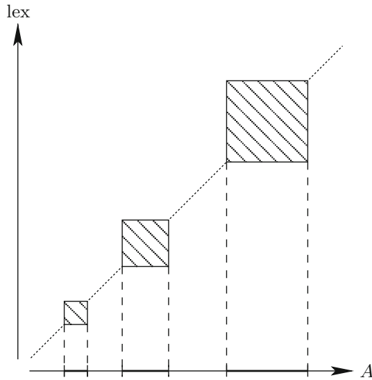
Figure 4.1: A high-level illustration of the order A used in the proofs of Theorem 3.2 and Lemma 4.2 . The horizontal axis contains the binary strings ordered under A , and the vertical axis represents the rank of the strings in the lexicographic order. The ranks in the two orders ( A and \text{lex} ) are identical (thus yielding in this \text{lex} -rank plot the dotted line going from bottom left to top right), except for those strings belonging in the intervals \mathcal{I}(x) (for x \in \Sigma^* ), which locally deviate from the lexicographic order (depicted as shaded boxes in the figure and as thick intervals on the A -axis).
