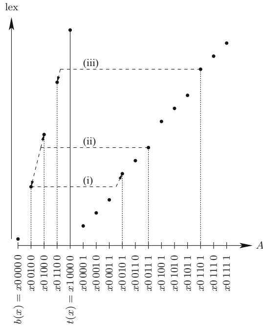
Figure 4.2: Example of an interval \mathcal{I}(x) in the proof of Lemma 4.2. The horizontal axis contains the strings of \mathcal{I}(x) ordered under A , and the vertical axis represents the rank of the strings in the lexicographic order. For this particular x , all computation paths of M(x) have length 3. The only paths that appear in M(x) are \{000, 010, 100, 110\} . The following calculations of \tilde{z} or of \tilde{z}^- and \tilde{z}^+ are illustrated: (i) for z = x00100 , \tilde{z} = x00101 (Case 1 of the proof of Lemma 4.2), (ii) for z = x00111 , \tilde{z}^- = x00100 and \tilde{z}^+ = x01000 (Case 2 of the proof of Lemma 4.2 when y = 011 does not correspond to a computation path), and (iii) for z = x01101 , \tilde{z}^- = \tilde{z}^+ = x01100 (Case 2 of the proof of Lemma 4.2 when y = 110 corresponds to a computation path).
