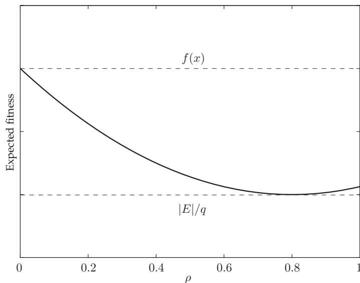
Figure 2: Expected fitness of an offspring of x , that is, E(f(M_\rho(x))) , plotted against mutation rate \rho for the graph coloring problem. The fitness of the current solution x is denoted by f(x) , whereas |E|/q is the average fitness over all solutions.
