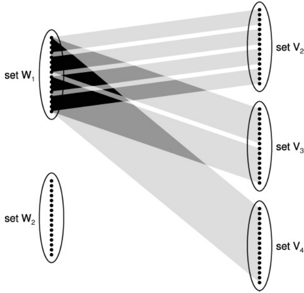
Figure 1: An illustration of Graph 1 for k = 4 . The gray straps should indicate complete bipartite subgraphs. For better clarity, the edges incident to W_2 are omitted.
