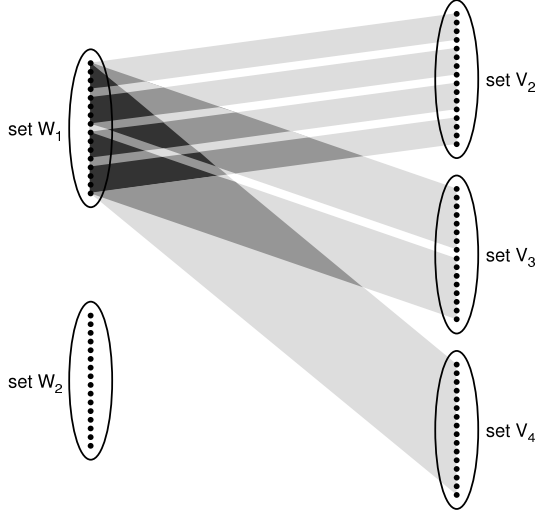
Fig. 1. An illustration of Graph 1 for k = 4 . The grey straps should indicate complete bipartite subgraphs. For better clarity, the edges incident to W_2 are omitted.
