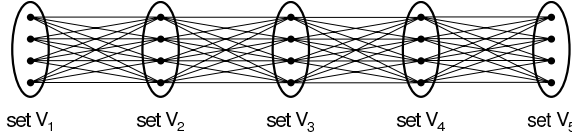
Fig. 3. An illustration of Graph 3 for k = 4 .
