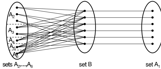
Fig. 2. An illustration of Graph 2 for k = 6 .
