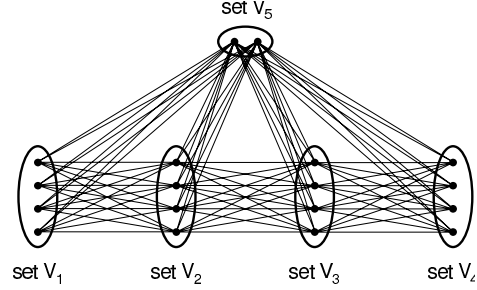
Fig. 4. An illustration of Graph 4 for k = 4 .
