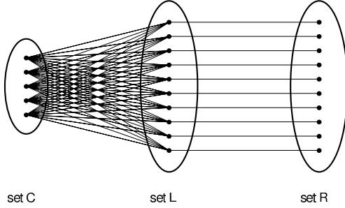
Fig. 5. An illustration of Graph 5 for k = 10 and \ell = 5 .
