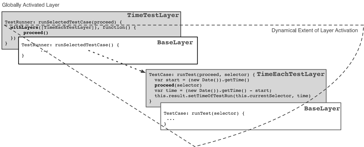
Fig. 4. The refined runSelectedTestCase method activates the TimeEachTestLayer and thus refines runTest of the class TestCase for the dynamic extent of this execution.
