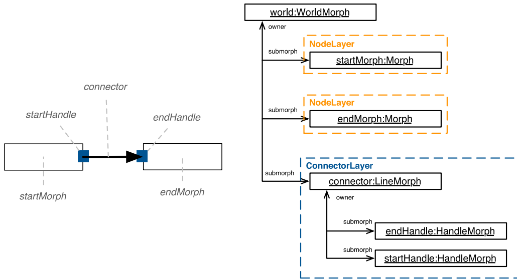
Fig. 5. A Morphic scene graph of the connector example. Both startMorph and endMorph have instance-specific NodeLayer activations. startHandle and endHandle are in the structural scope of the ConnectorLayer which is explicitly activated only in the connector.
