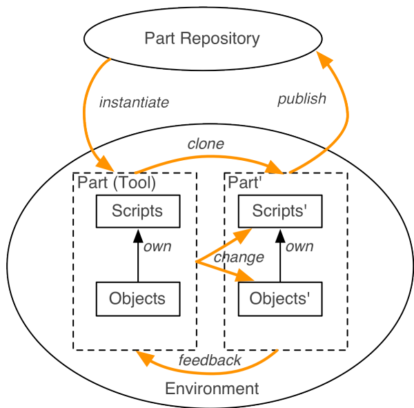
Figure 6: Flow of changes and feedback in a system were changes are encapsulated in scoped layers
