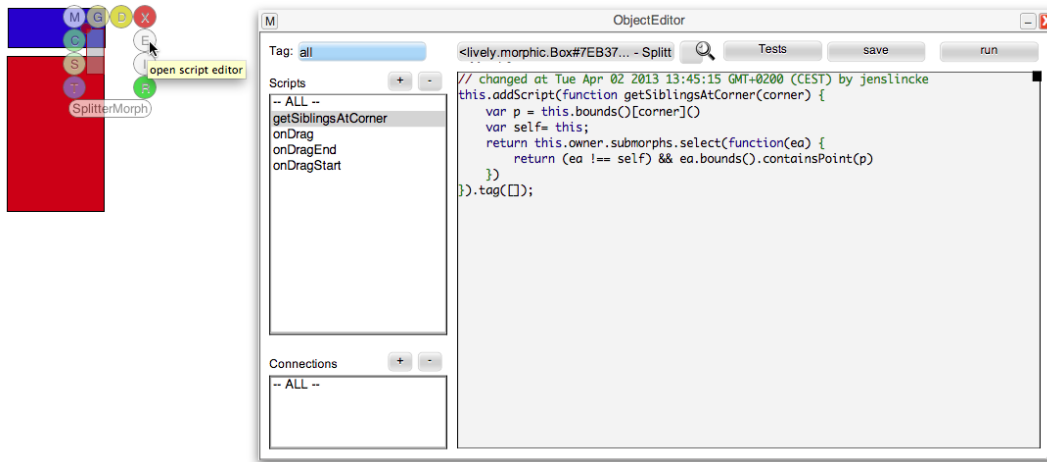
Figure 8: Editing the SplitterMorph with Halo and ObjectEditor
