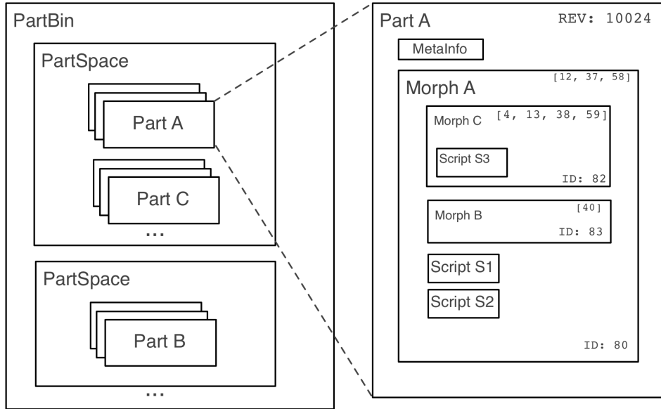
Figure 4: Morphs are serialized as Parts, grouped in PartSpaces inside the PartsBin
