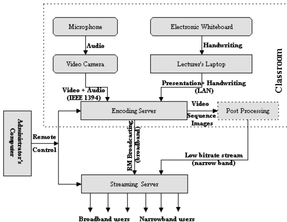
Figure 1 System Structure
