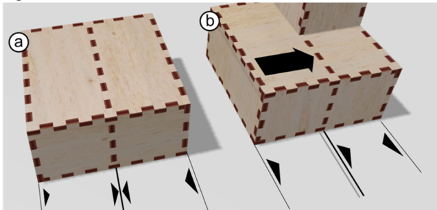
Figure 17: (a) When applying the reinforcement tool to this part, the reinforcement centers itself, (b) However, when adding a boxel, reinforcement automatically shifts by half a plate thickness so as to line up with the left plate of the added boxel, producing a sturdier result.
