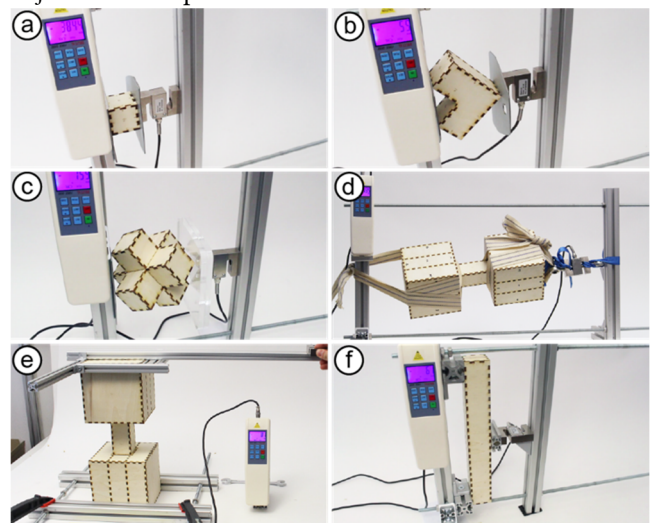
Figure 23: The test apparatus.
