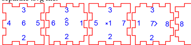
Figure 4: An exported model from Kyub, the red lines are what the laser cutter cuts. Numbers along the edges tell users which plates (numbers in centers) to connect to, when assembling the model. A ‘^’ indicates “this side up”; an ‘x’ indicates placement at the bottom.
