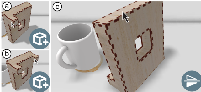
Figure 7: Add boxel remains applicable after the use of deformation tools.
