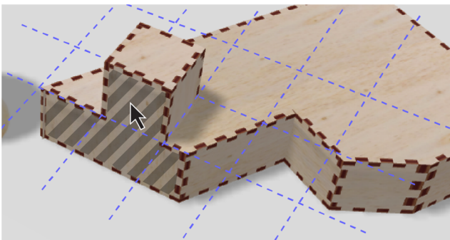
Figure 28: The resulting boxel is merged with the assembly. The dashed surface is an example of a coplanar plate that is unified with the side of the added boxel.
