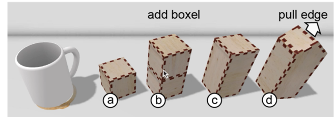
Figure 2: Kyub allows users to create sturdy objects by stacking volumetric elements, which we call boxels. (a) A single boxel can withstand >500kg of load, (b) Added boxels merge automatically, resulting in a larger, yet equally strong structure. (c) While kyub offers the affordance of a voxel-based editor, its objects are not bound to a grid; users can reshape them using a wide range of deformation tools.
