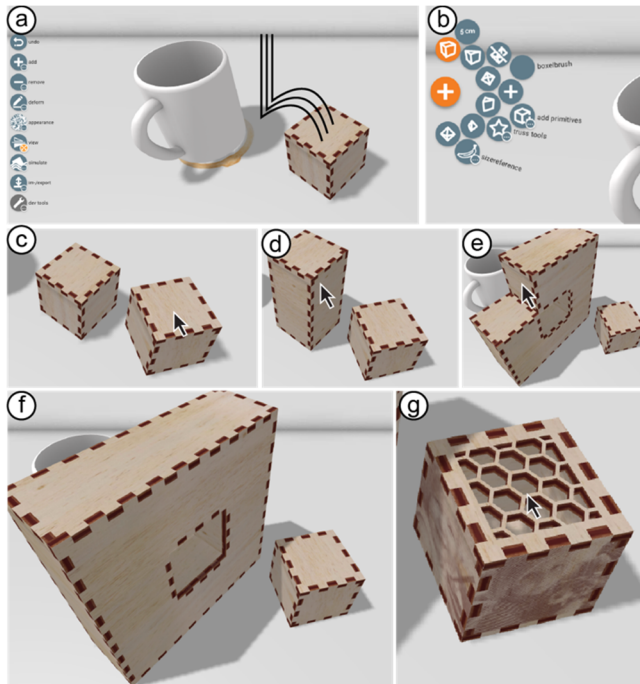
Figure 3: Sole use of the add boxel tool already allows making simple objects, here a picture frame. (a) A boxel falls into the scene. (b) The user selects add boxel and (c) clicks the stage, which produces a second boxel. (d) Holding the add boxel tool, the user clicks a boxel already on stage. This stacks a boxel on top and both merge automatically. (e) Adding another six boxels (f) completes the frame. (g) Engraving six images into the lone boxel prepares it for being displayed in the frame.
