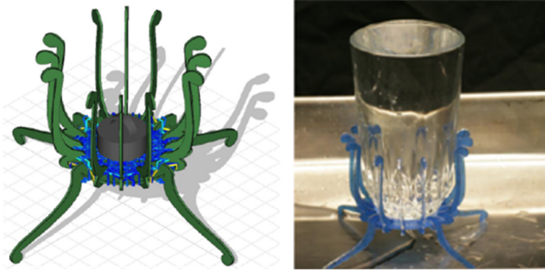
Figure 21: A glass holder made using FlatFitFab [6] holding up a glass of water weighing 275 grams.
