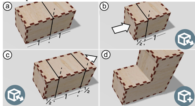
Figure 8: Kyub infers the grid, rather than maintaining it (a) Laying down two boxels, (b) pushing in half a boxel and (c) pulling out half a boxel on the other side results in 2x1 boxel arrangement. (d) Adding a boxel snaps into position based on the current shape of the part, not its history.
