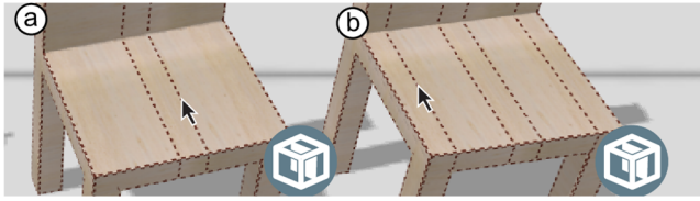
Figure 16: (a) Chair with front-to-back reinforcement, (b) additional reinforcement supporting the legs.
