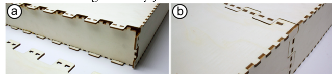
Figure 19: The cell structure created by tessellation. The big finger joints lock the two coplanar plates on the top while supported by a vertical plate.
