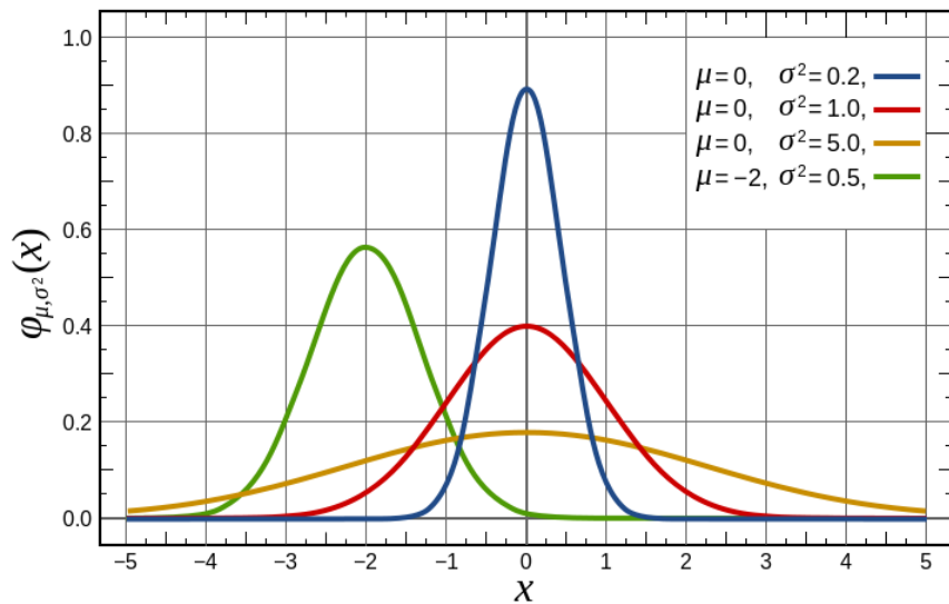
Normal distributions
