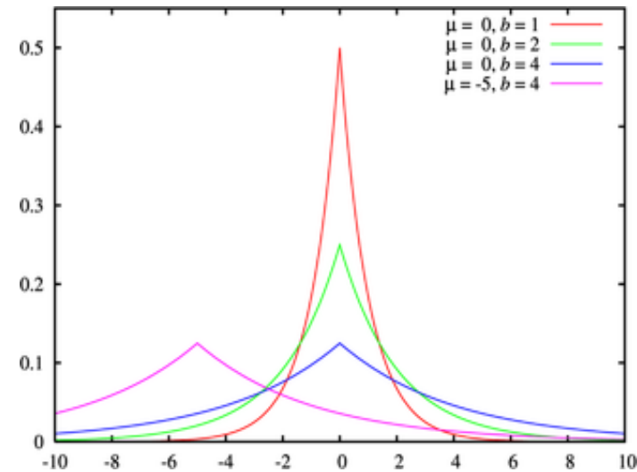
Laplace distributions
