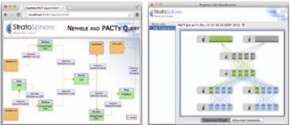
Figure 1: Top: Meteor's Query Submission Interface. Bottom left: Optimized PACT plan. Bottom right: Nephel execution graph.
