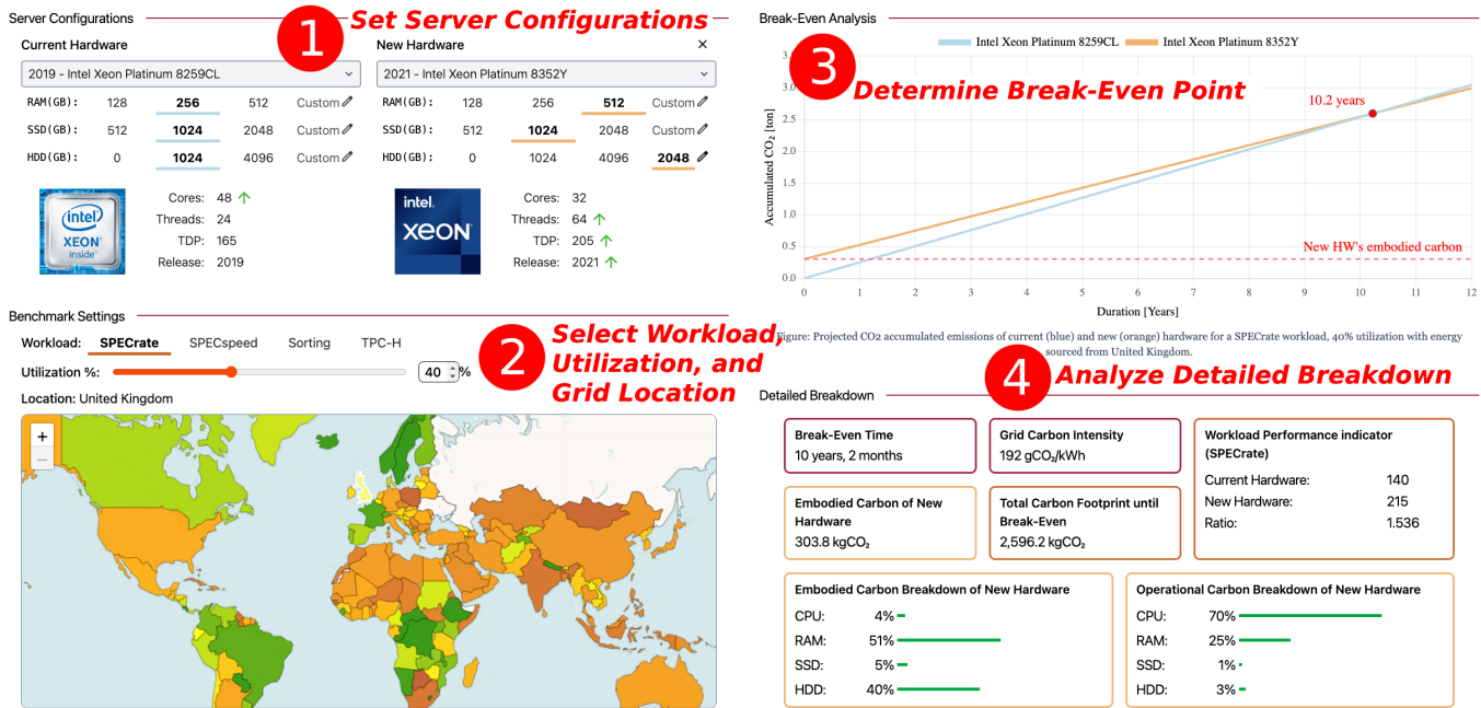
Figure 2: The user interface of TCO 2 .
