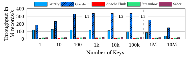
Figure 11: Throughput for scaling the state size.
