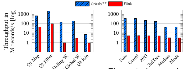
Figure 8: Aggregation functions.
