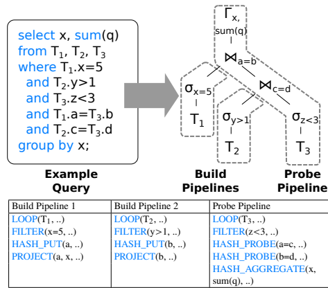
Fig. 2: Segmentation of example query into pipeline programs.
