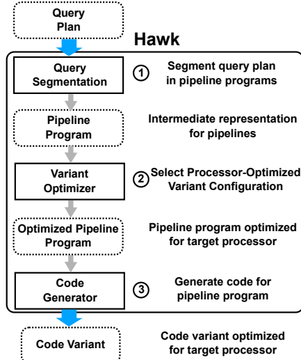
Fig. 1: Hawk’s compilation process.
