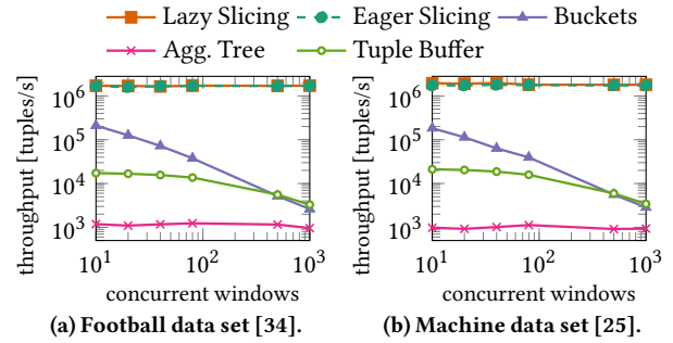
Figure 9: Increasing the number of concurrent windows including 20% out-of-order tuples and session windows.
