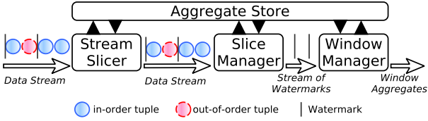
Figure 7: The Stream Slicing and Aggregation Process
