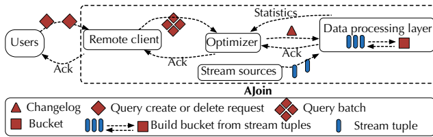
Figure 3: AJoin architecture
