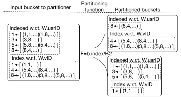
Figure 9: Example partitioning of the bucket described in Figure 4e
