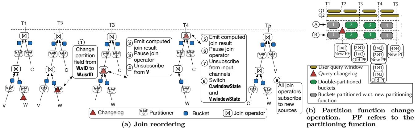
Figure 12: Run-time QEP changes: Join reordering (left) and partitioning function change (right)
