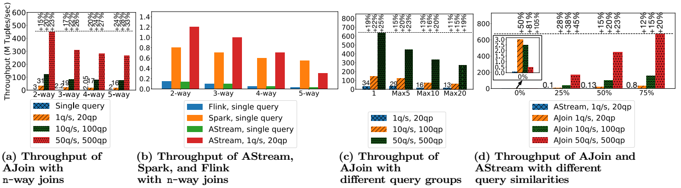
Figure 20: Throughput measurements for AJoin, AStream, Spark, and Flink. +P% above the dashed lines denote that the throughput increases by P% when queries are submitted at compile-time.
