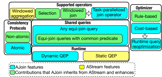
Figure 2: Comparison between AJoin and AStream
