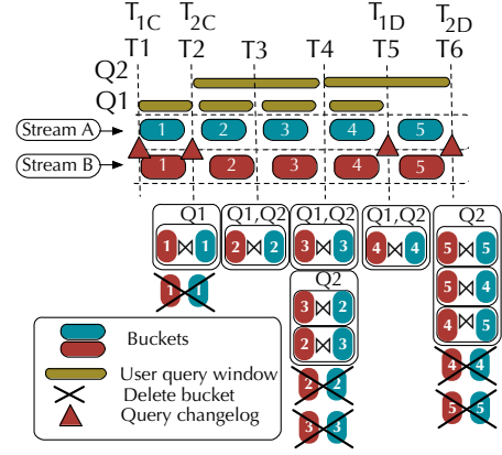
Figure 8: Ad-hoc join example. The join operation is performed between T1C and T2D .
