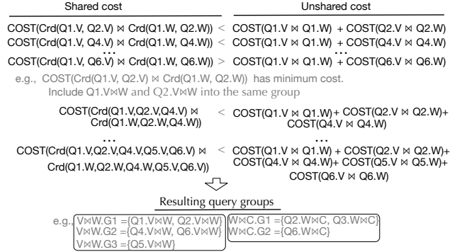
(a) Calculation of query groups
