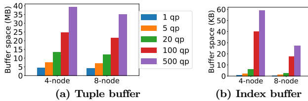
Figure 16: Buffer space used for tuples and indexes inside a 1-second bucket
